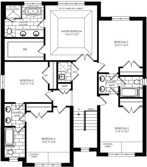
Elevation A Optional Second Floor 5 Bedroom Plan
