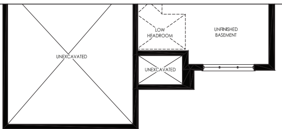
Elevation B Basement
