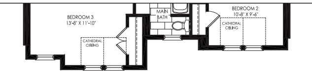
Elevation B Second Floor
