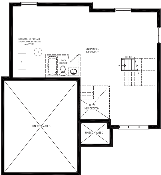
Elevation A & B Basement
