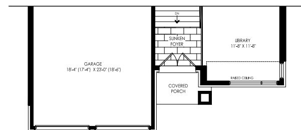
Elevation C Ground Floor
