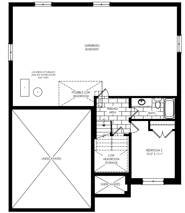
Elevation A Basement
