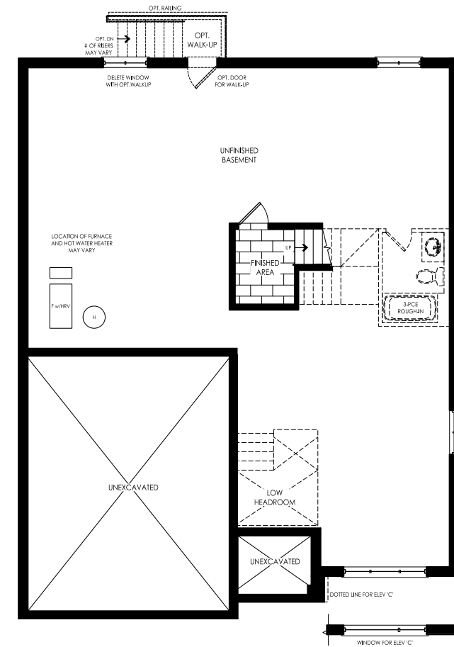
Elevation A, B & C Basement
