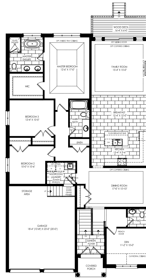
Elevation A Optional Ground Floor
