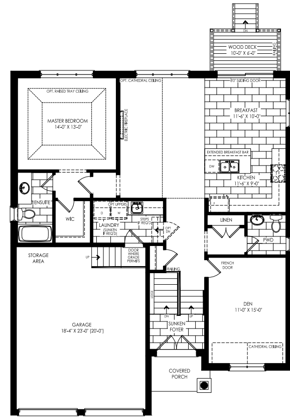
Elevation A Ground Floor
