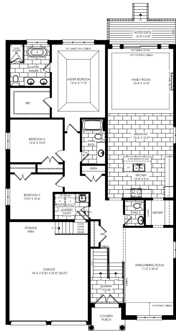
Elevation A Ground Floor
