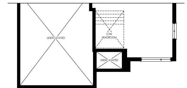
Elevation C Basement
