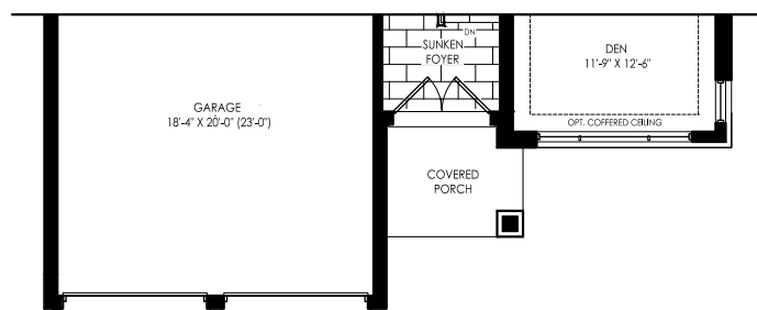
Elevation C Ground Floor
