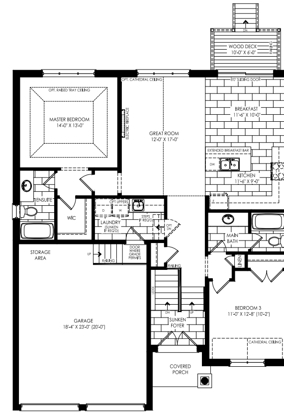
Elevation A Optional Ground Floor with 3 Bedrooms
