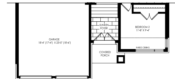
Elevation C Optional Ground Floor with 2 Bedrooms
