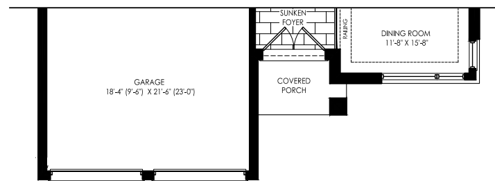
Elevation C Ground Floor
