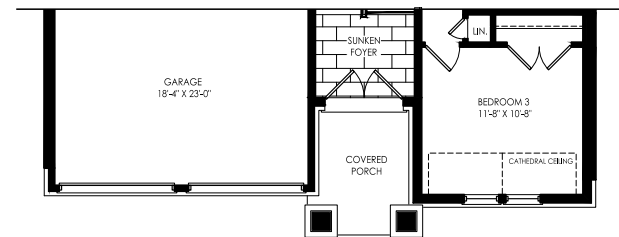
Elevation B Ground Floor
