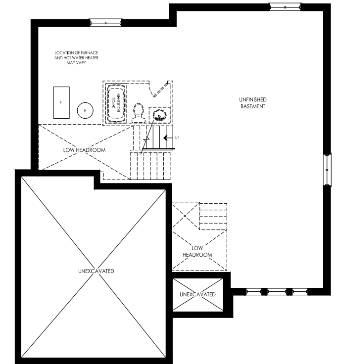
Elevation A Basement
