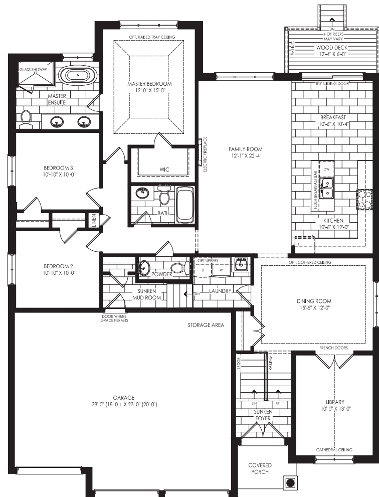
Elevation A Ground Floor
