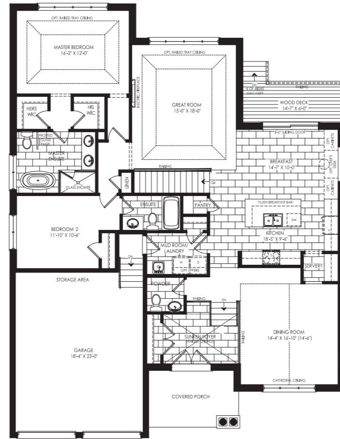
Elevation A Ground Floor
