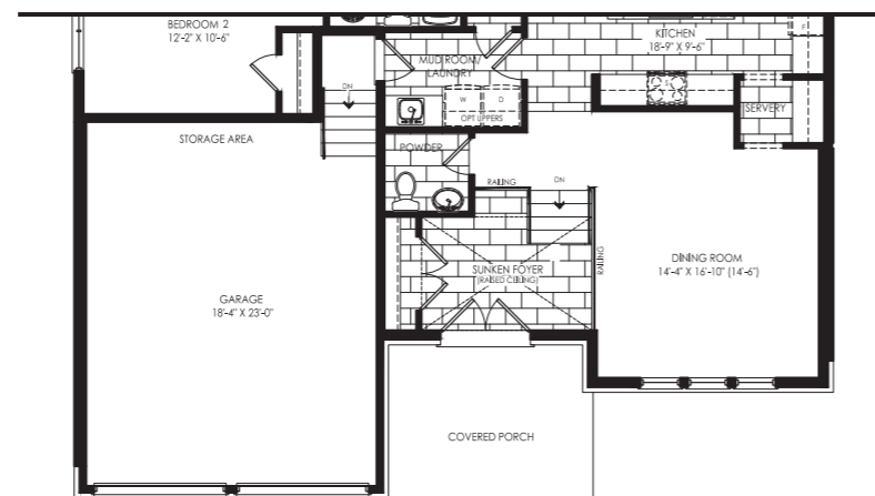
Elevation B Ground Floor
