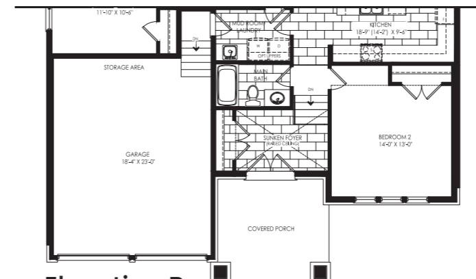
Elevation B Optional Ground Floor with 3 Bedrooms
