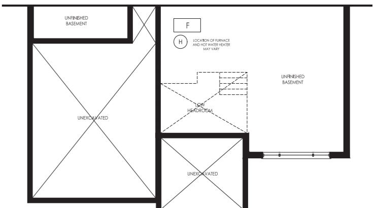
Elevation C Basement
