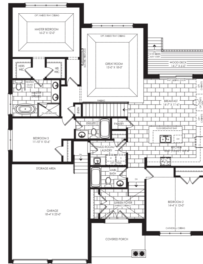
Elevation A Optional Ground Floor with 3 Bedrooms
